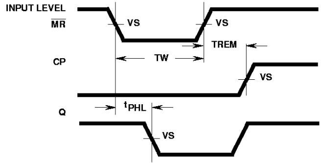
FIGURE 2. MASTER RESET PULSE WIDTH, MASTER RESET TO OUTPUT DELAY AND MASTER RESET TO CLOCK RECOVERY TIME
